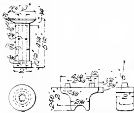
Figs. 4876-7. AXLE SAFETY-STRAP THIMBLE. Figs. 4878-9. TRANSOM TRUSS-ROD SEAT.
